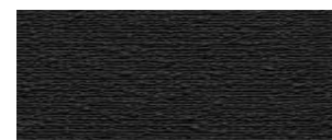
T-02 Graphite
